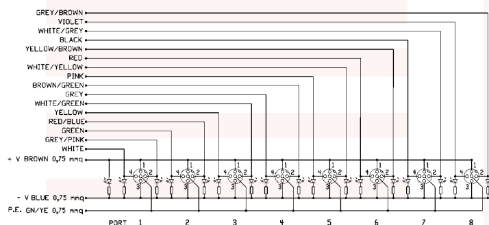
8 Outputs 5 Poles
