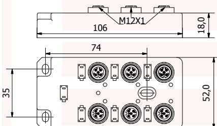
6 Outputs 5 Poles
