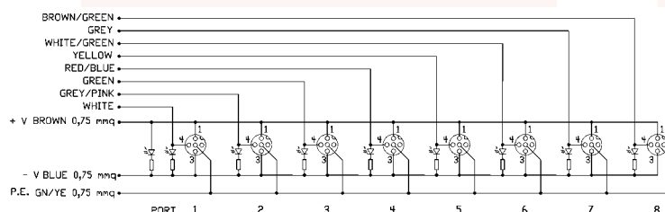
8 Outputs 4 Poles
