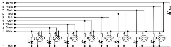
8 Outputs 3 Poles
