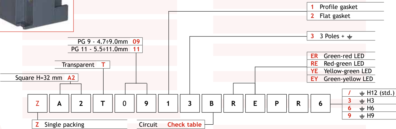
Connectors for pressure switches with double LED indicator
