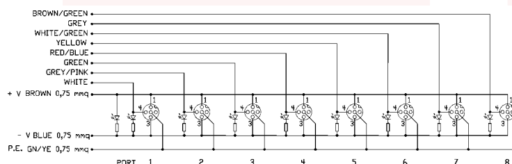
8 Outputs 4 Poles
