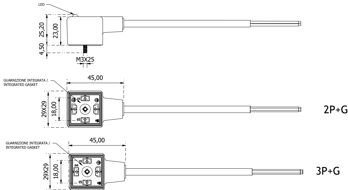
AB2 - AB3 series with or without circuitry
