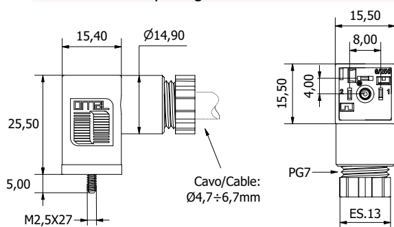
C1 series cable gland size PG7 Spacing 8 mm
