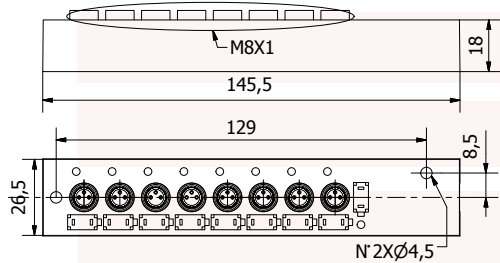
8 Outputs 3 Poles
