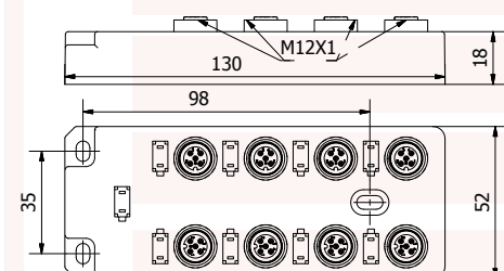
8 Outputs 5 Poles
